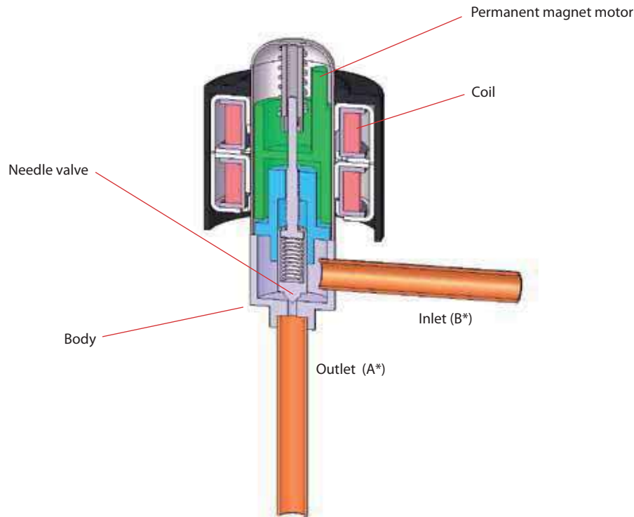
Cross section diagram of ETS 6 series
