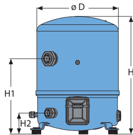
MT / MTZ / NTZ 2 cylinders
