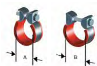
Hose collars for Hose Whip Restraint System
